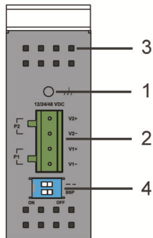
Top Panel View
