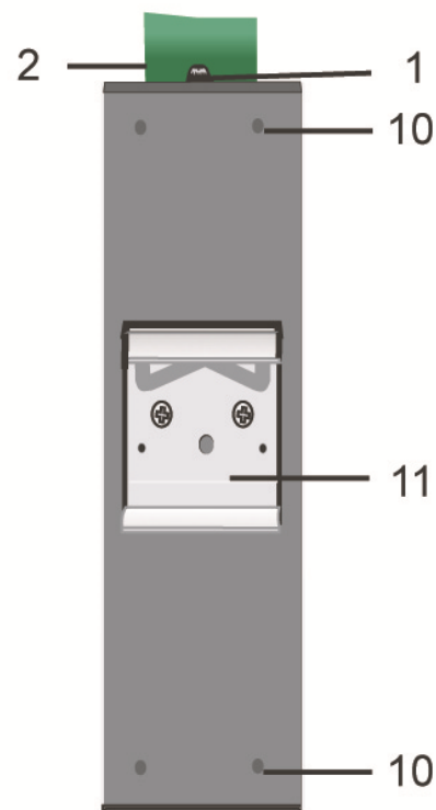
Rear Panel View
